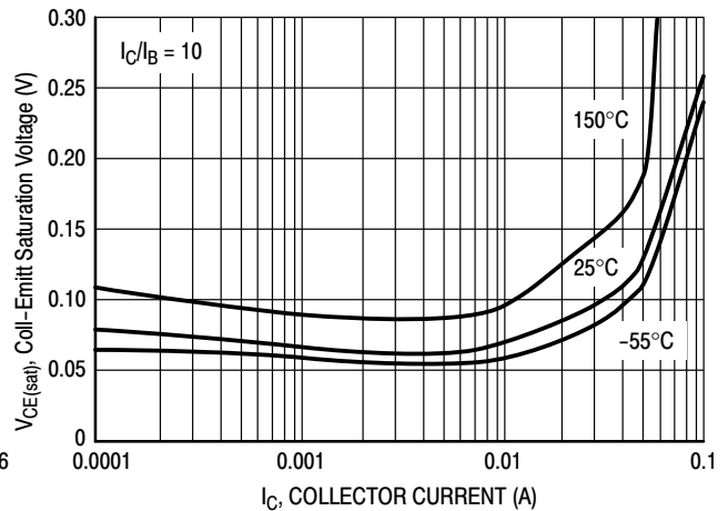
Figure 4. V_{CE(sat)}
