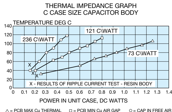
Thermal Impedance Graph with Ripple Current
